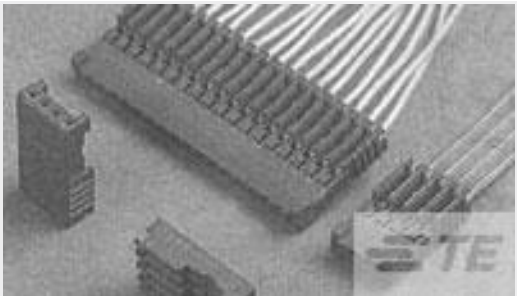
TE 产品编号281786-5 PLUG HE14 IDC 180 5 P AWG 28-26
