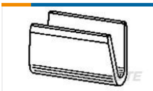
TE 产品编号160725-1 SPLICE 26-22 AWG .008 PTPB
