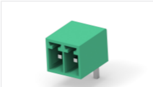
TE 产品编号2350514-2 2POS TB HDR 90 DEG, PITCH 3.5 & TL 3.5mm
