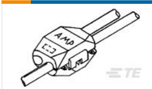
TE 产品编号53440-1 ELECTRO-TAP, 18-14 AWG RUN&TAP
