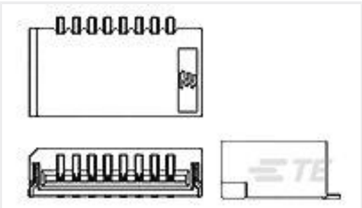
TE 产品编号3-84981-0 1MM FFC SMT H ASSY 30P EMBOSS
