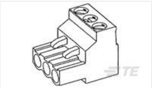
TE 产品编号282808-4 TERMI-BLOK PLUG STACKING 4P.10
