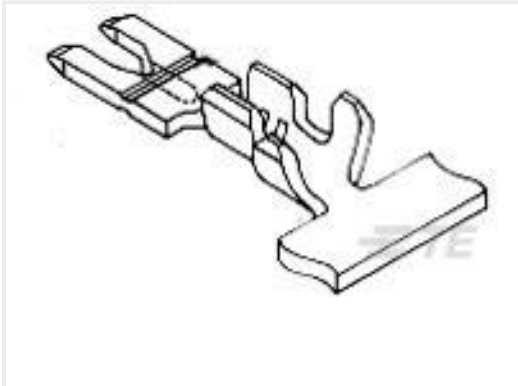
TE 产品编号281622-2 MAG-MATE TAB STD SNPL
