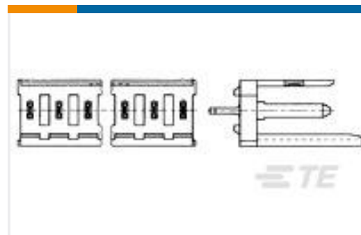
TE 产品编号280609-1 2P MOD 1 SHROUDED HEADER, ST, TIN PLTD
