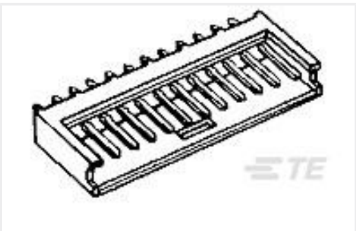
TE 产品编号280371-1 4P AMPMODU II SHRD HDR, ST, TIN
