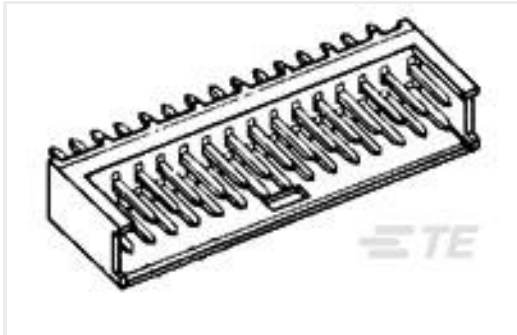
TE 产品编号280385-1 2X8P AMPMODU II SHRD HDR, ST, TIN
