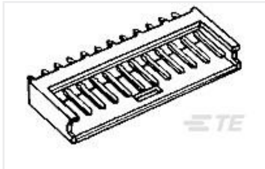
TE 产品编号280374-1 10P AMPMODU II SHRD HDR, ST, TIN
