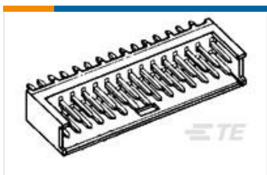
TE 产品编号280384-1 2X4P AMPMODU II SHRD HDR, ST, TIN
