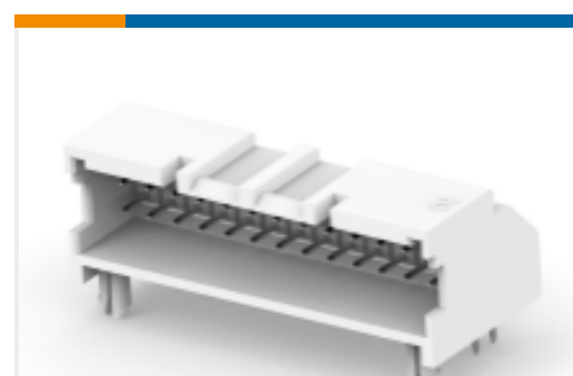
TE 产品编号2-2323750-6 ASSY,HDR,RIGHT ANGLE,GWT,DUAL ROW, EP2.5
