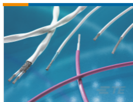
TE 产品编号647612-000 2 Core Twisted Pair Cable: Tin Coated Copper Cable, 20 AWG
