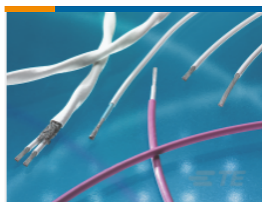
TE 产品编号069794-000 2 Core Twisted Pair Cable: Silver Coated Cable, 24 AWG
