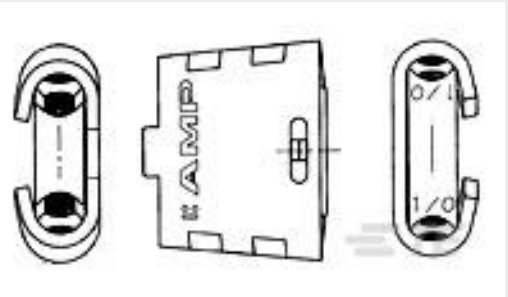
TE 产品编号83592-6 MINIWEDGE,SYM,#2-#4,CORE
