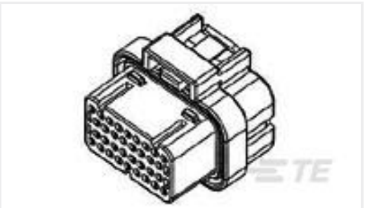
TE 产品编号1473712-1 SUPER SEAL 2ROW 26POS PLUG ASS
