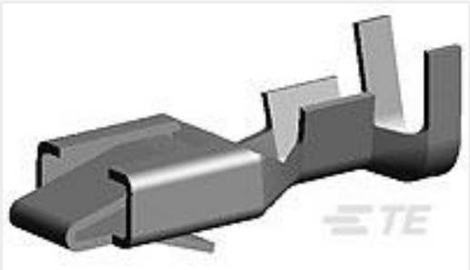
TE 产品编号640417-2 BLADE REC 250 18-14AWG TPBR
