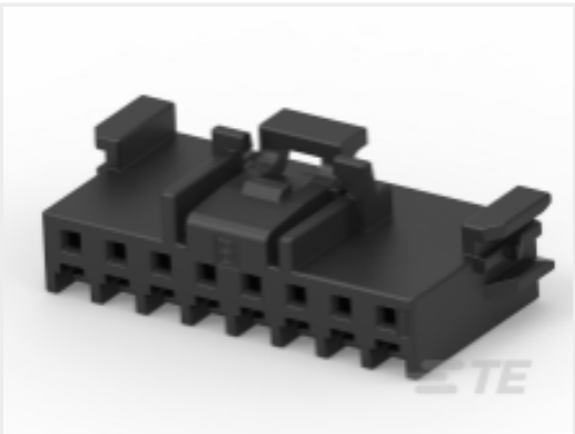
TE 产品编号 2-2350224-8 SGI 2.0 Plug Housing, 8 Position, Key B
