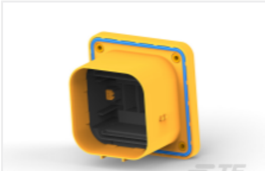
TE 产品编号2315855-6 MSD,REC HSG ASSY,630A,V0,M8
