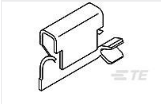
TE 产品编号63733-3 GROUND CLIP 18-22AWG TPPBR
