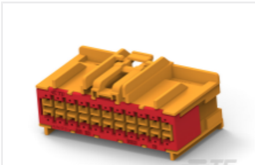
TE 产品编号2300979-1 22POS,0.64 GENER. Y,REC HSG ASSY, COD A
