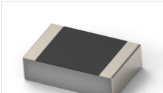
TE 产品编号2176452-6 CPF 0201 604R 0.1% 25ppm 1K RL
