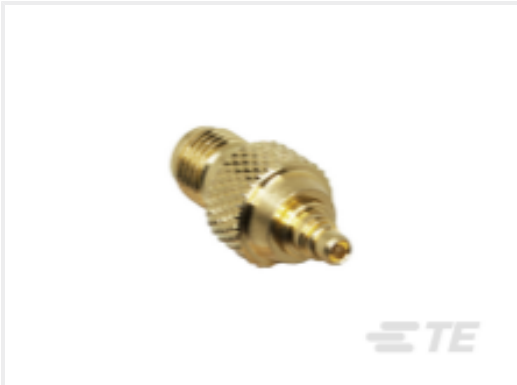
TE 产品编号ADP-SMAF-MMXM SMA Jack to MMCX Plug
