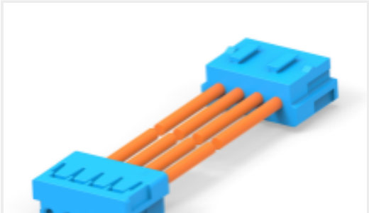
TE 产品编号2405869-4 CT 4P 300MM CABLE ASSEMBLY 2-179228-4
