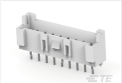
TE 产品编号2404280-9 EP 2.5 HDR, GLOW WIRE, 9P
