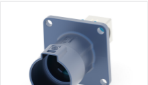
TE 产品编号CAT-AQ4-HHD1400180 PowerTube HVP-HD 1400 180° 接头
