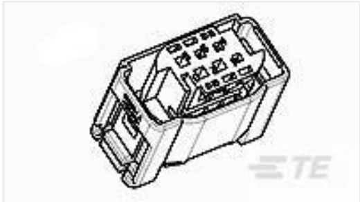
TE 产品编号1-967640-1 4POS MQS REC COD A
