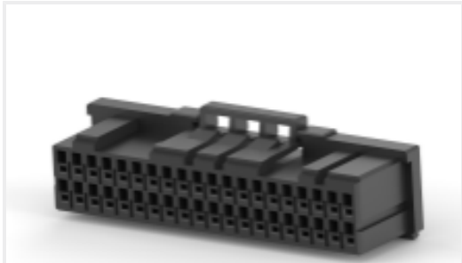
TE 产品编号1-2333134-0 DYNAMIC 1100D REC HSG X 40P BLACK 33%GF
