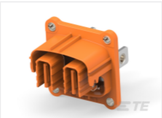
TE 产品编号2405532-2 2POS,PCON18,HDR ASSY,COD A
