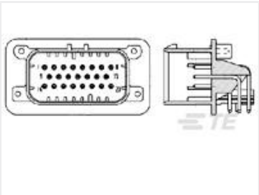
TE 产品编号1-776087-4 23POS,PIN DIA 1.3,HDR ASSY,90DEG, COD 4
