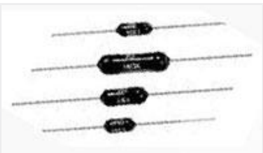
TE 产品编号5-1879659-1 H4 3K83 0.1% 15PPM
