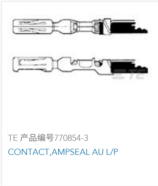
TE 产品编号770854-3 CONTACT,AMPSEAL AU L/P
