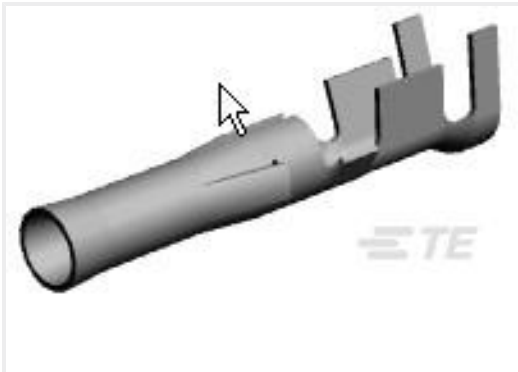
TE 产品编号770144-1 .093 CP&S SOK PTPBR L/P 20-14
