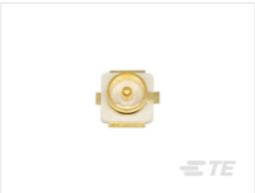
TE 产品编号CONUFL001-SMD-T U.FL/MHF1 Jack 50 Ohm PCB Surface Mount
