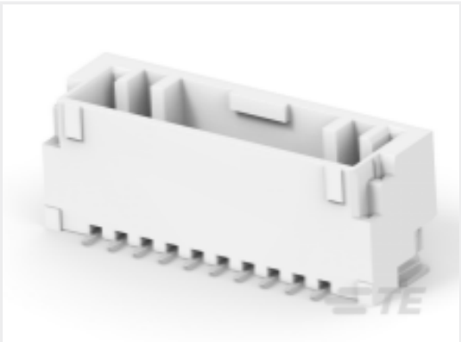
TE 产品编号1-2360540-0 SGI 1.25 HDR, 10P, VT, Key A, Natural
