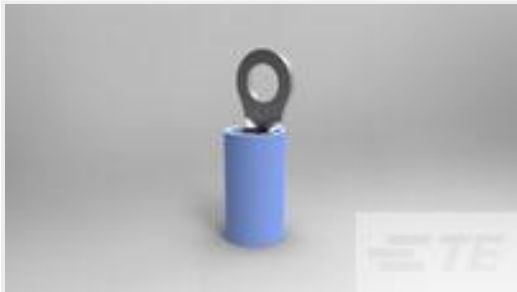
TE 产品编号32442 TERMINAL,PIDG R 16-14 6
