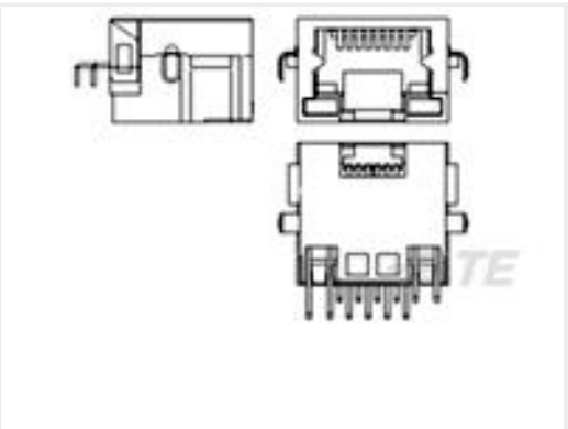
TE 产品编号2041126-1 MODULAR JACK, RJ45, SMT TYPE,AU: 6u"
