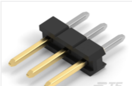
TE 产品编号2355172-4 4P,2MM,BRK HDR,SRVT,2.8,0.1AU,BOX
