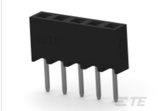
TE 产品编号 2307769-5 5P,2MM,B-B,REC,SRVT,3.2,0.1AU,TUBE
