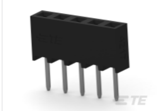
TE 产品编号 2307767-5 5P,2MM,BB,REC,SRVT,2.0,0.1AU,TR,W/CP
