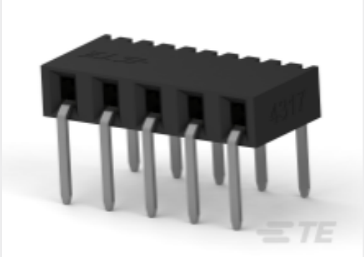
TE 产品编号 2314928-5 5P,2MM,B-B,REC,SRHZ,2.1,0.1AU,TB
