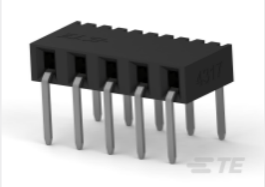
TE 产品编号 2307704-5 5P,2MM,B-B,REC,SRHZ,2.8,0.1AU,TB
