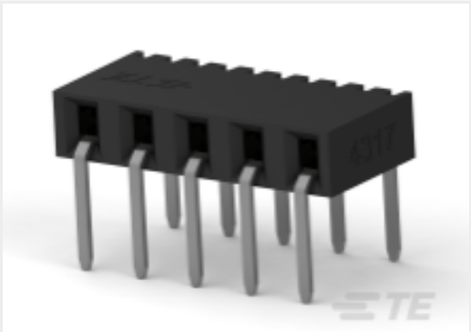
TE 产品编号 2307705-5 5P,2MM,B-B,REC,SRHZ,3.4,0.1AU,TUBE
