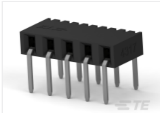
TE 产品编号 2314936-5 5P,2MM,B-B,REC,SRHZ,2.8,0.1AU,TR
