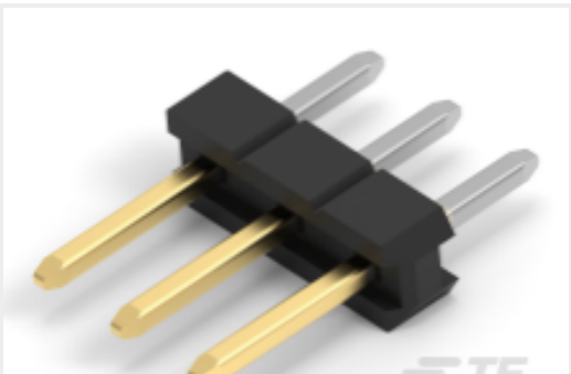
TE 产品编号2355172-3 3P,2MM,BRK HDR,SRVT,2.8,0.1AU,BOX
