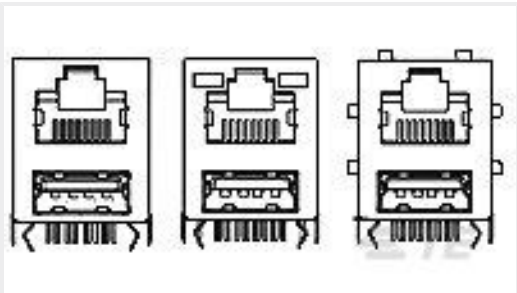
TE 产品编号1775855-1 Modular Jack RJ45 stacked over USB
