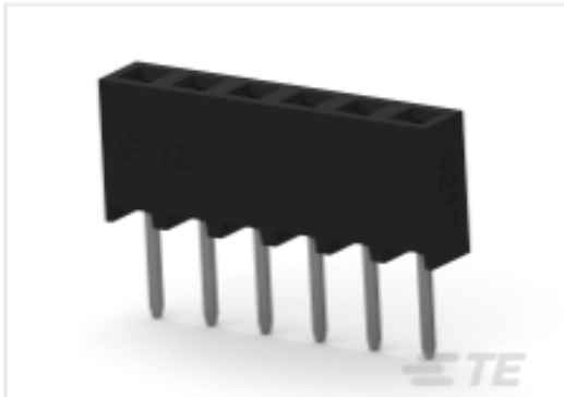
TE 产品编号 2314876-6 6P,2MM,B-B,REC,SRVT,2.7,0.1AU,TB
