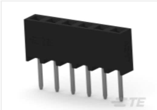
TE 产品编号 2314880-6 6P,2MM,BB,REC,SRVT,2.7,0.1AU,TB,W/CP
