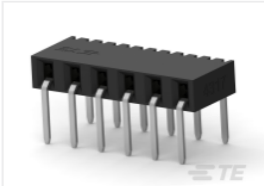
TE 产品编号 2307704-6 6P,2MM,B-B,REC,SRHZ,2.8,0.1AU,TB
