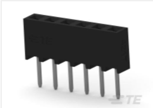
TE 产品编号 2307767-6 6P,2MM,BB,REC,SRVT,2.0,0.1AU,TR,W/CP
