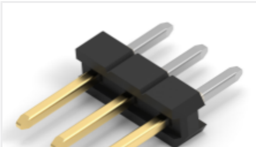
TE 产品编号2355045-3 3P,2MM,BRK HDR,SRVT,2.8,0.1AU,TB
