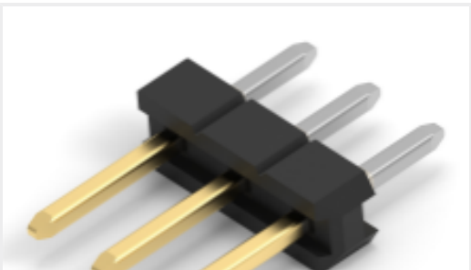
TE 产品编号2355045-4 4P,2MM,BRK HDR,SRVT,2.8,0.1AU,TB
