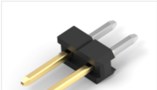
TE 产品编号2355045-2 2P,2MM,BRK HDR,SRVT,2.8,0.1AU,TB
