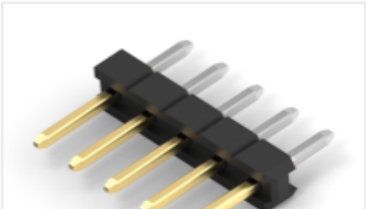
TE 产品编号2355104-6 6P,2MM,BRK HDR,SRVT,2.8,0.1AU,TB W/CAP
