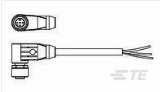
TE 产品编号2273099-3 M12 x 1.0 angled socket pigt shld A
