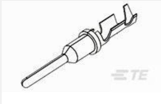
TE 产品编号1924463-3 PIN, SF, SIZE 16, 18-20 AWG, NI/SN
