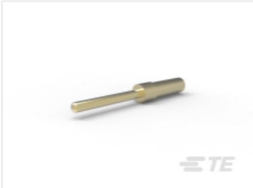
TE 产品编号2334110-2 PIN CRIMP CONTACT AWG 20-24
