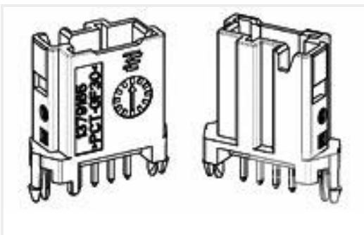
TE 产品编号1379165-7 4pos MQS .63 header 180deg THR
