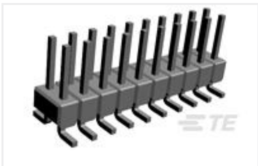
TE 产品编号1-1241050-0 2x10P MOD II BREAK AWAY HDR, SMD, BLISTER
