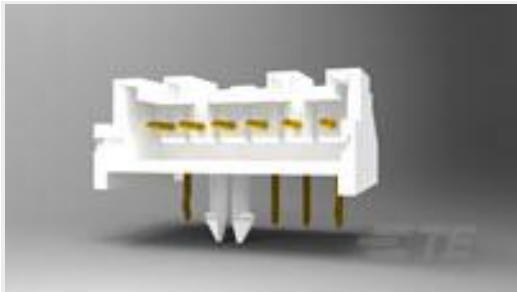
TE 产品编号1744426-7 Header Housing Assy, EP 2.5 RA, 7 Pos.
