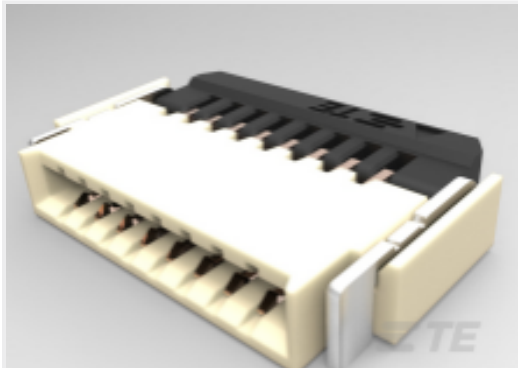
TE 产品编号2328702-8 8PIN 0.5MMP FPC CONNECTOR, BACK FLIP LOCK
