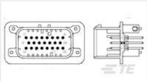
TE 产品编号1-776231-4 35POS,PIN DIA 1.3,HDR ASSY, 180DEG,COD 4
