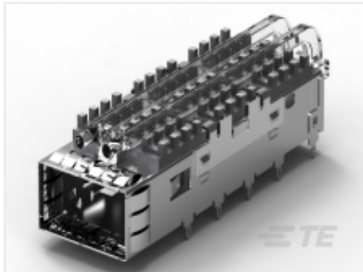
TE 产品编号 2-2170705-7 CAGE ASSY, QSFP28 1X1, SPRING, HS, LP
