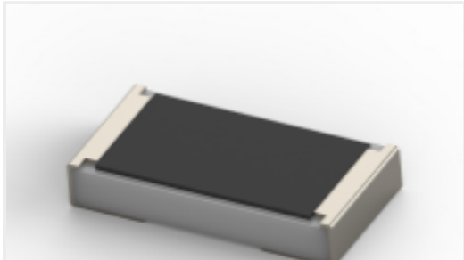
TE 产品编号2176469-3 TLRP 2010 2.0W R030 1% 75PPM 4K RL
