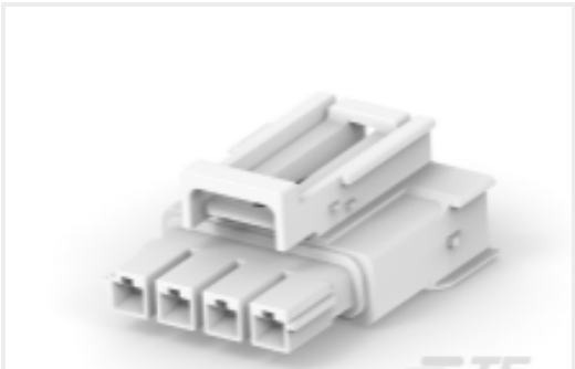
TE 产品编号2329913-1 PWR VERSA-LOCK RECPT, 14-16 AWG
