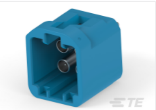
TE 产品编号2378550-3 4P MATE-AX HDR,ASSY , 180deg, COD C
