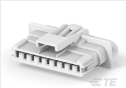
TE 产品编号2443729-9 PLUG HOUSING SDL2.5 WATERPROOF 9PIN
